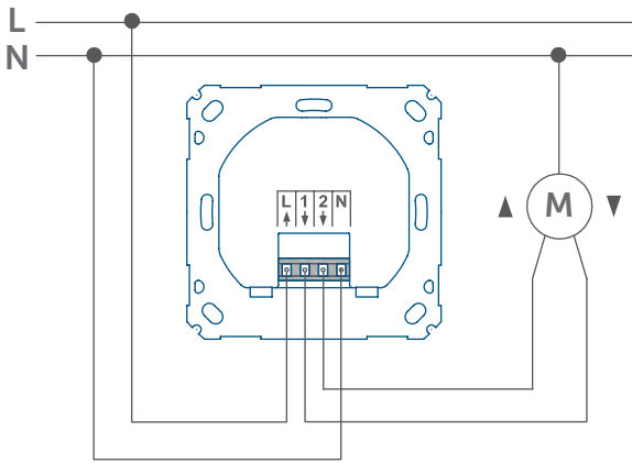
For installation of the shutter actuator, a neutral conductor is required.
